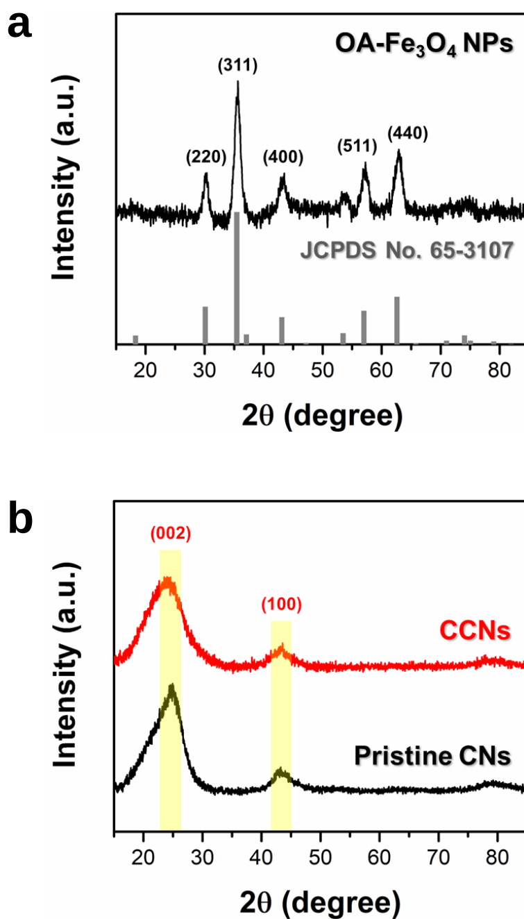
Figure S1. a) XRD patterns of synthesized OA-Fe 3 O 4 NPs (top) with referential cubic spinel-structured Fe 3 O 4 crystals (bottom; JCPDS card No. 65-3107). [S4] b) XRD patterns of interface-modified CCNs (top) and pristine CNs (bottom).
