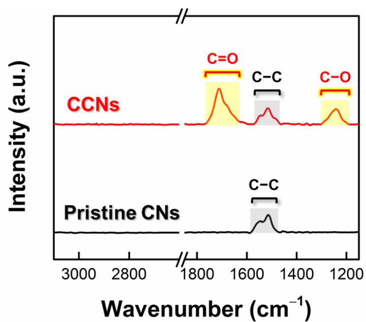
Figure S2. FTIR spectra of interface-modified CCNs (top) and pristine CNs (bottom).
